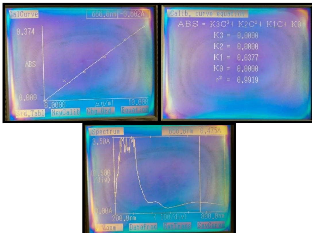
Image No.1: Calibration curve & calibration equation of Gallic acid
