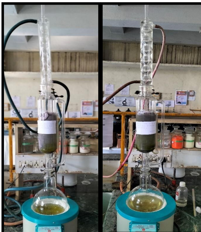
Image No.10: Soxhlet Extraction Ethyl acetate and Methanol Extraction
