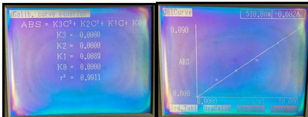
Image No.17: Calibration curve & calibration equation of Quercetin
