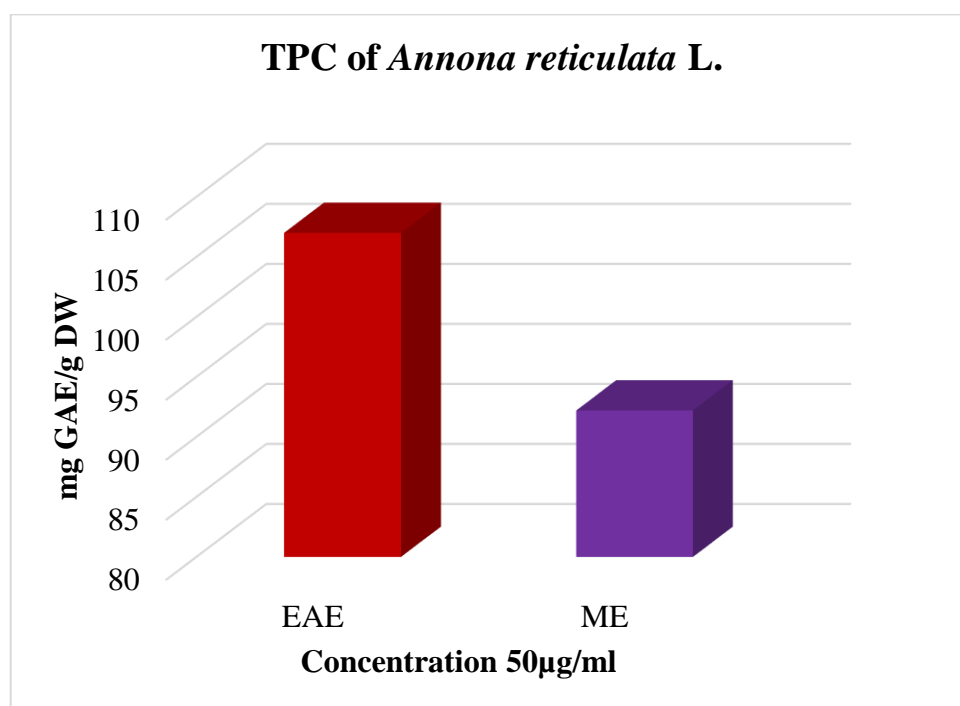
Graph No.1: TPC of Annona reticulata L.
