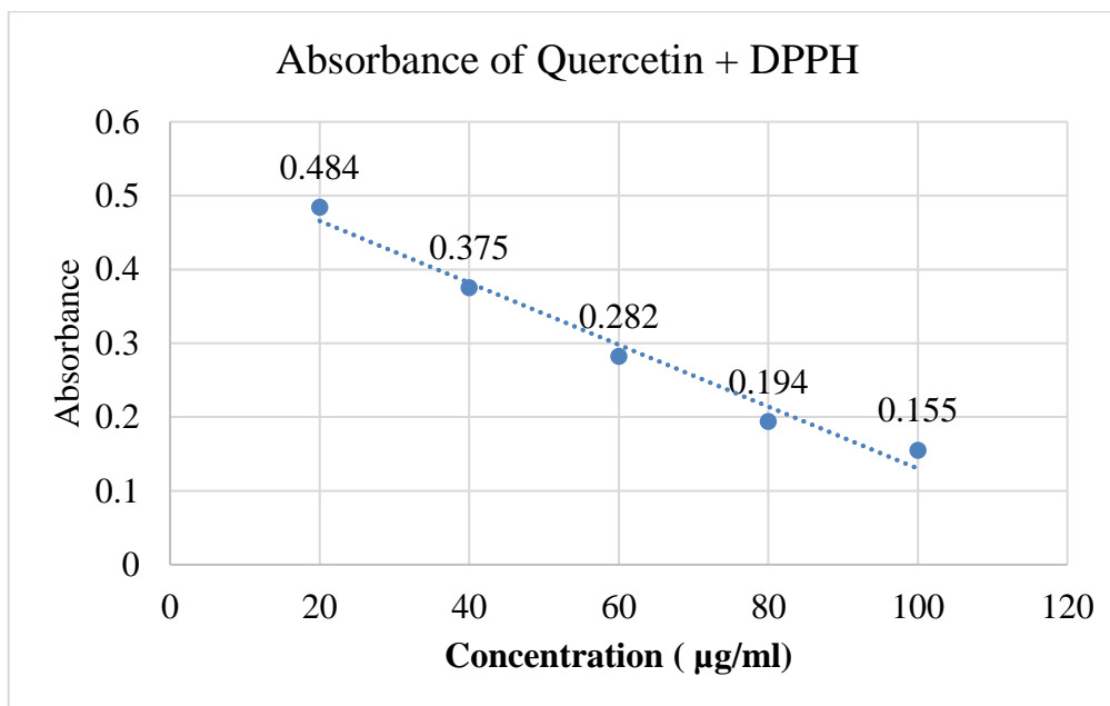
Graph No.3: Absorbance of Quercetin + DPPH
