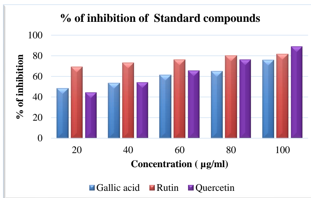
Graph No.4: % of inhibition of Standard compounds
