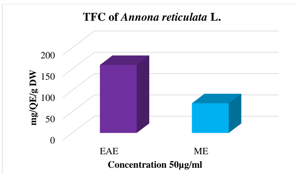
Graph No.2: TFC of Annona reticulata L.
